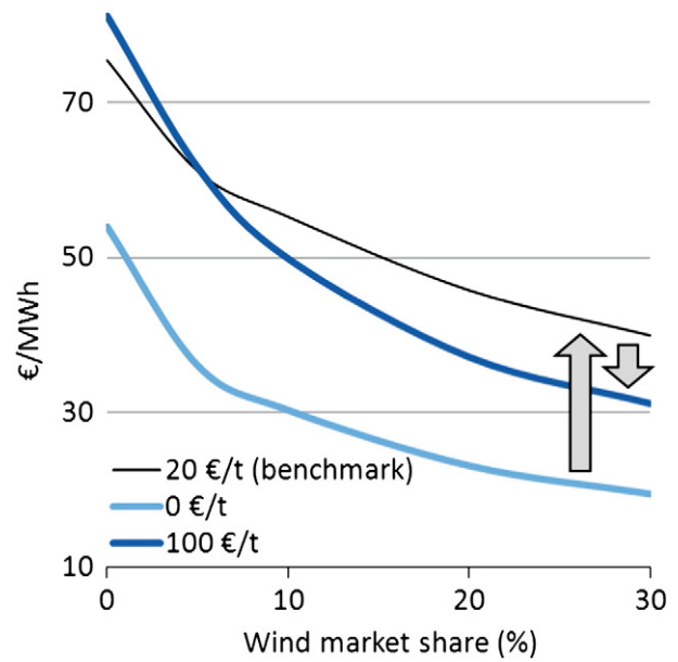
Fig. 21. Absolute long-term wind value at different CO 2 prices. At penetration rates above 5%, a CO 2 price of 100€/t results in lower income for wind generators than 20€/t. The arrows indicate the change in income as the CO 2 rises.
