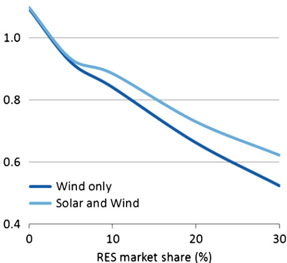
Fig. 16. Wind value factor with and without solar.
