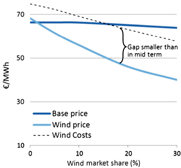
Fig. 19. The long-term wind market value in absolute terms. While the value is twice as high as the mid-term value at high penetration rates, it is still significantly below full costs.
