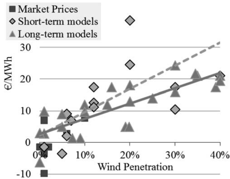
Figure 8: Wind Profile Cost Estimates for Thermal Power Systems
