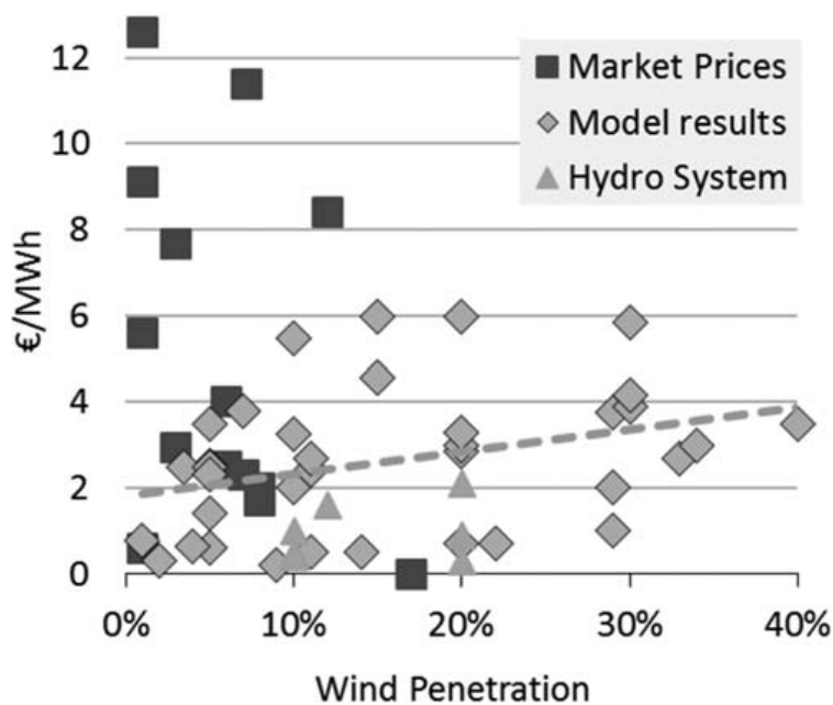
Figure 9: Wind Balancing Cost Estimates for Thermal Power Systems
