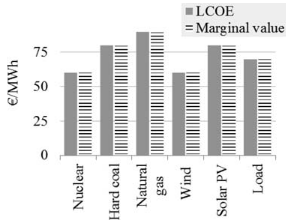
Figure 3: LCOE and Marginal Value in the Long-Term Optimum
